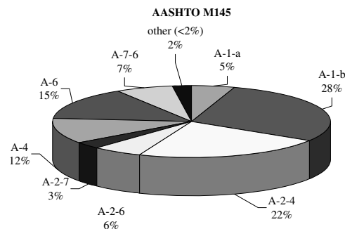
Figure 3. Schematic representation of the types of soils tested
