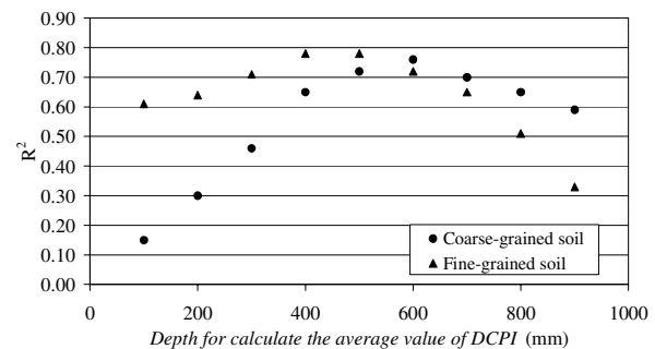
Figure 5. Coefficient of determination ( R^2 ) obtained for different depths
