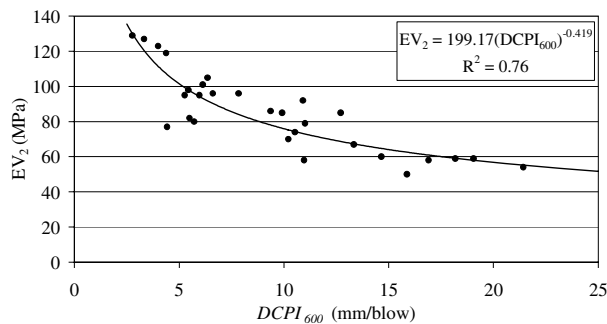
Figure 6. Relation between DCPI_{600} and EV_2 for coarse-grained soils
