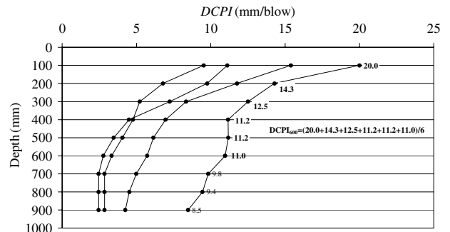
Figure 4. DCPI values obtained for different depths
