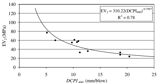
Figure 7. Relation between DCPI_{400} and EV_2 for fine-grained soils
