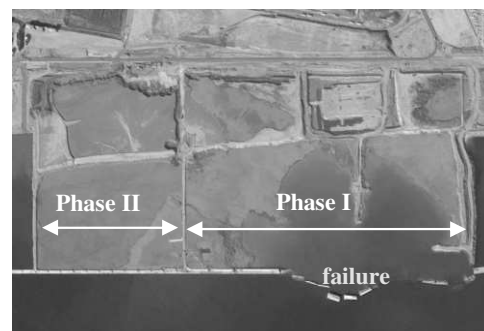
Figure 1. Aerial photo of phase I and II of the container terminal. Caisson failure partially affected Phase I (Courtesy of Barcelona Port Authority).
