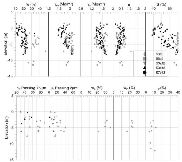
Figure 3. Fill properties in Phase I ("a" boreholes, grey symbols) and Phase II ("b" boreholes, black symbols).
