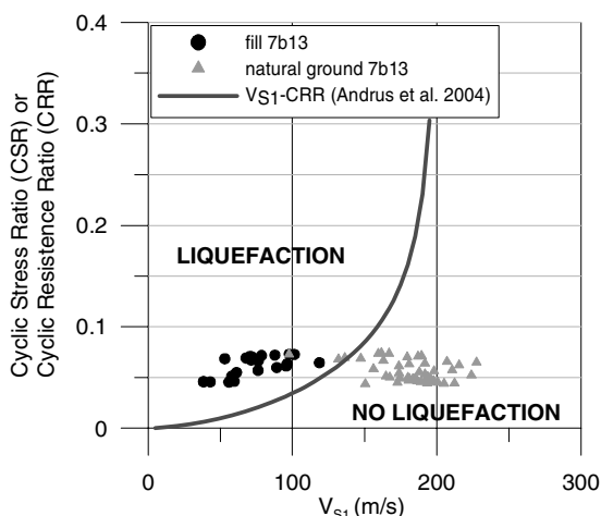
Figure 8. Assessment of the potential for liquefaction based on SDMT results. Test 7b13.
