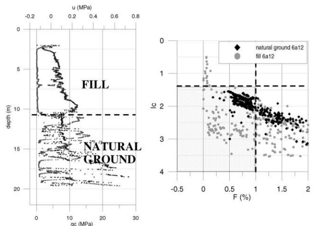
Figure 4. Results of the CPTu 6a12 test. The shaded area indicates sensitive material.
