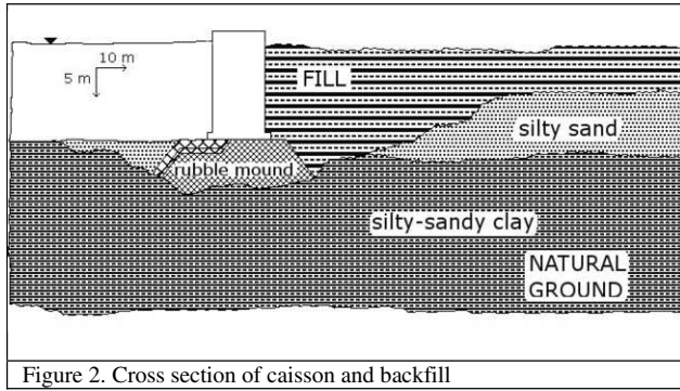
Figure 2. Cross section of caisson and backfill
