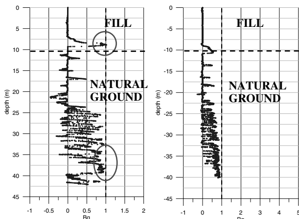
Figure 9. B_q values for cone test CPTu-5dp before preloading (left) and after preloading (right).
