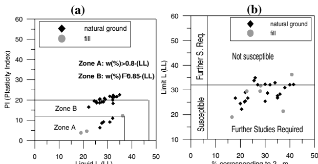
Figure 5. Identification of ‘liquefiable’ soil types. (a) Recommendations by Seed et al. (2003) (b) Criterion of Andrews & Martin (2000).
