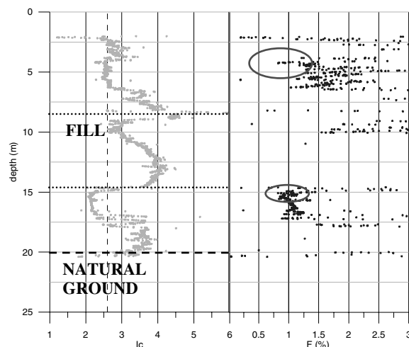
Figure 6. Application of ( I_c & F) liquefaction criteria for CPTU 6a8. Circled points indicate potential liquefaction
