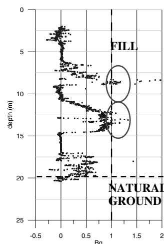
Figure 7. Application of B_q liquefaction criteria for CPTU 6a8 test. Circled points indicate potential liquefaction.
