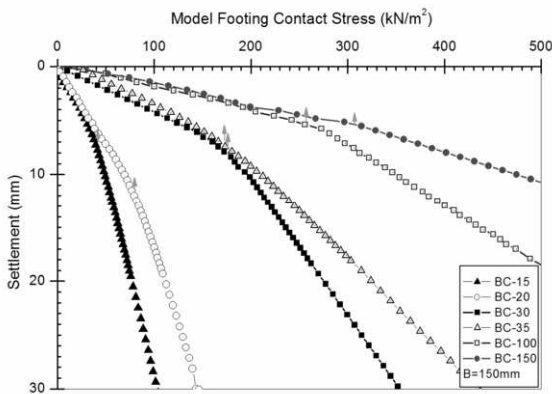
Fig. 4. Stress-settlement curves for Model Footing
