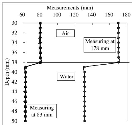
Figure 6. Comparison of measurements in the air and underwater
