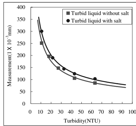
Figure 7. Effective range with various turbidities
