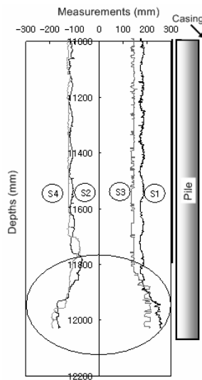
Figure 9. Results of field verification
