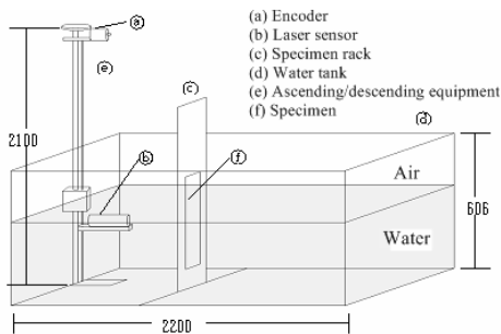
Figure 5. Laboratory verification System
