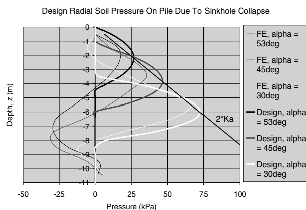
Figure 5. Comparison between finite element (FE) calculated and 'design' pressures on piles
