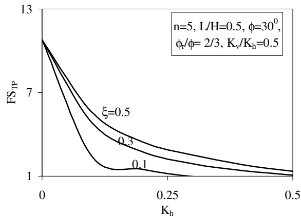
Fig. 8. Variation of Factor of Safety, FS_{TP} , with Horizontal Seismic Coefficient, K_h , - Effect of \xi ( =H/TV_s ).
