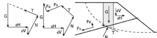
Figure 3. Contribution of soil nails to sliding resistance
