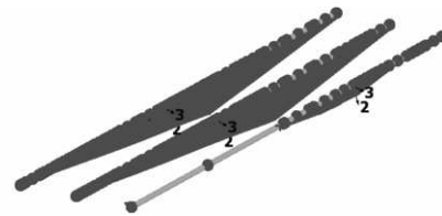
Figure 7. Normal forces and node distribution in nails indicating lower nail modelling problem
