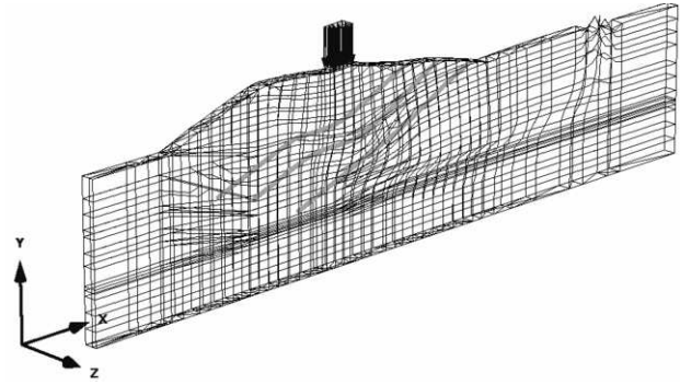
Figure 5. Deformed mesh with indication of deformation of the nails
