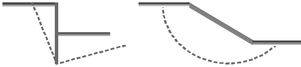
Figure 1. Preselected failure surfaces for classical ULS design.
