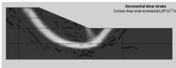
Figure 2. Failure surface indicated by band of high incremental shear strains.
