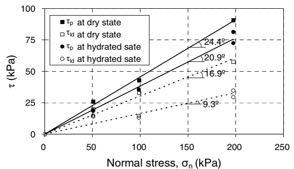
Figure 6. Shear strength envelopes for the GCL/GM interfaces
