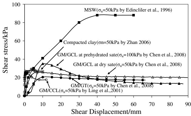
Figure 4. Shear stress-displacement relationships for MSW, compacted clay and interfaces within composite liners
