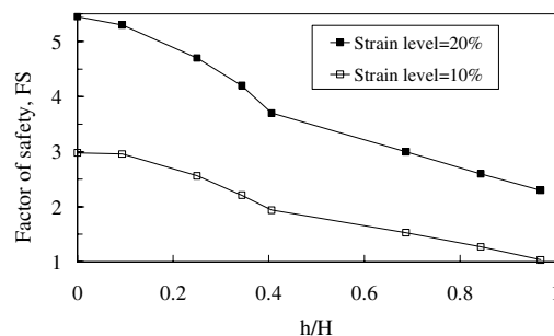
Figure 3. Influence of leachate level on the slope stability of the Suzhou landfill
