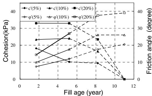
Figure 2. Relationships of shear strength parameters to the fill age of MSW (Zhan et al. 2008)
