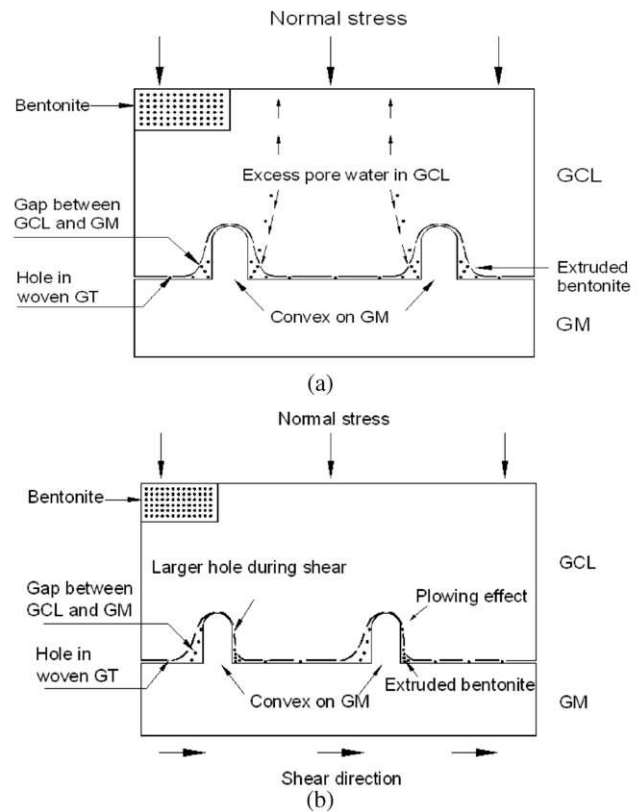
Figure 5. Bentonite extrusion mechanism of GCL: (a) Excessive pore-water pressure during rapid loading; (b) Plowing effect during shearing
