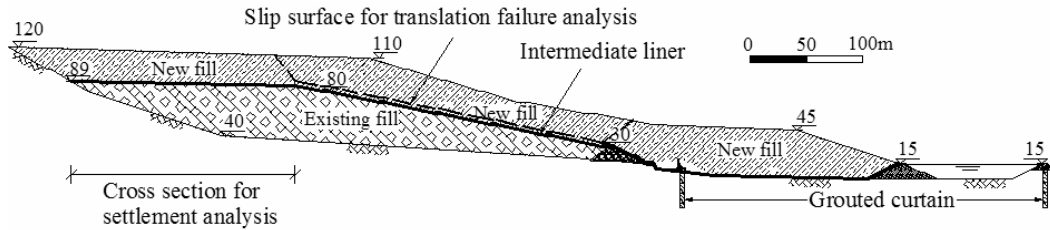
Figure 1. A preliminary design of landfill expansion in Suzhou, China
