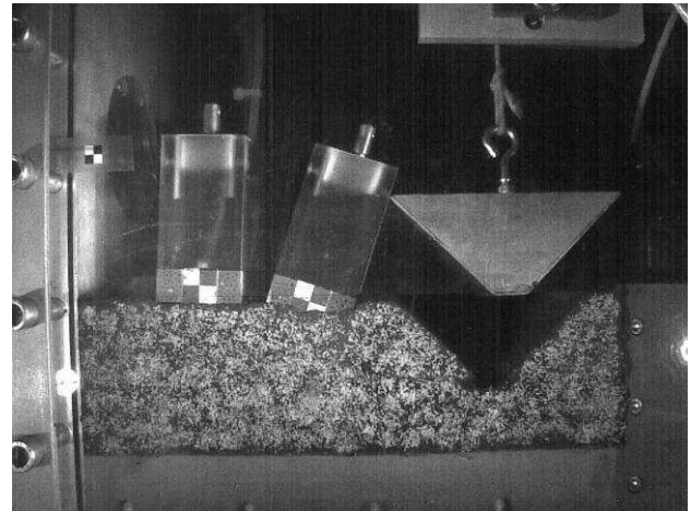
Figure 6. Centrifuge test representing the preliminary test
