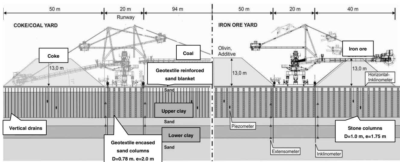
Fig. 4: Basic concept at the raw material yard; right side: stone columns under stock piles and runway corridor.
