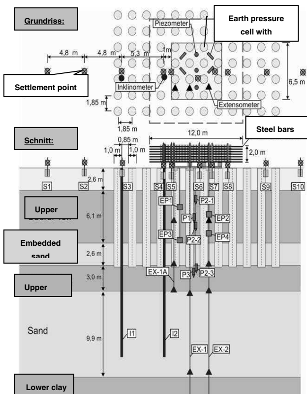
Fig. 7: Layout of large scale load test and instrumentation.
