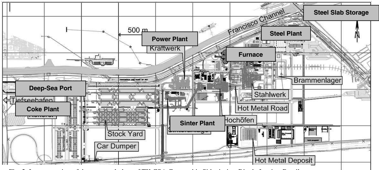
Fig. 2: Layout section of the new steel plant of TK CSA Companhia Siderúrgica, Rio de Janeiro, Brazil
