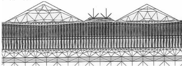
Fig. 6: Deformation prediction at runway corridor by FE-analysis.
