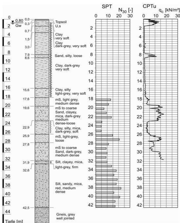
Fig. 3 (left): Typical subsoil profile for the raw material yard.
