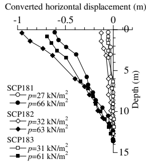
Figure 3. Distribution of horizontal displacement of improved ground
