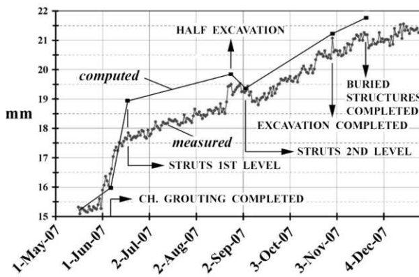
Figure 5. Gavotti Palace's vertical settlements comparisons, as measured on-site by the leveling system (jagged lines) and as computed by the FEM analysis (straight lines).
