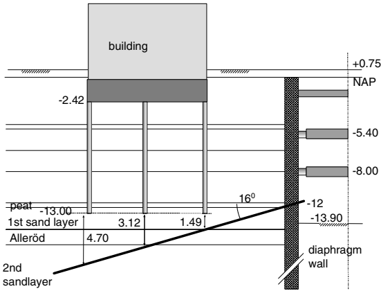
Figure 2. cross-section location. Dimensions in m.
