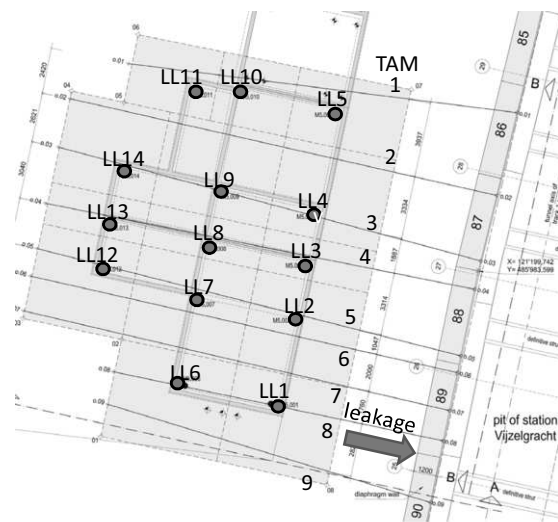
Figure 1. Top view of corrective grouting location, Vijzelgracht.
