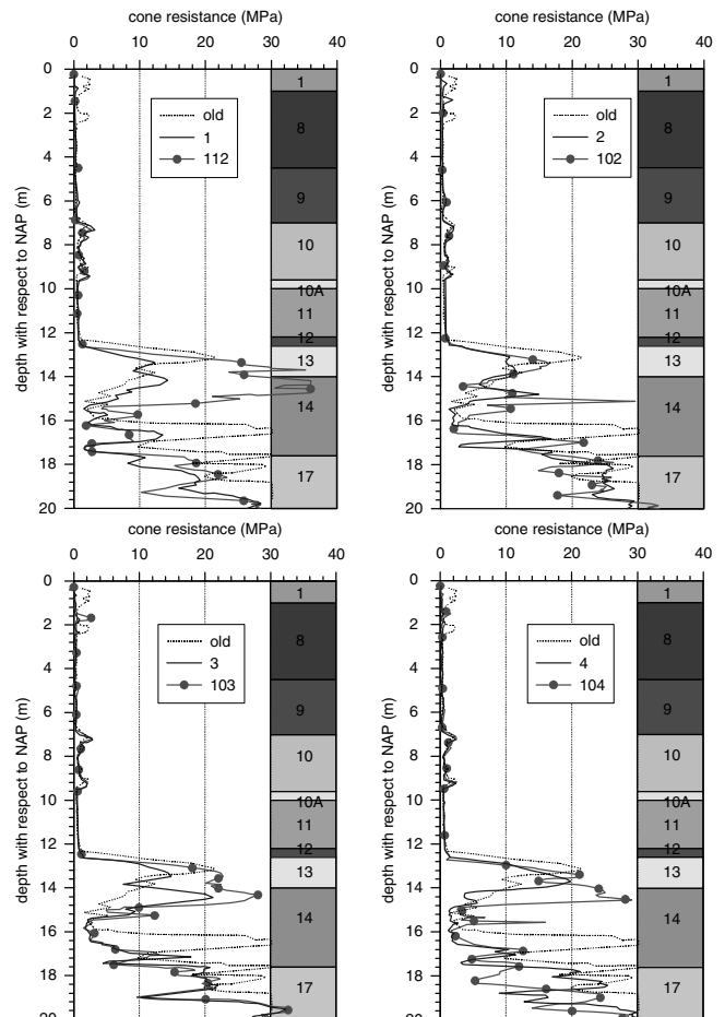
Figure 4: CPTs for location 1, to 4 before (1 - 4) and after (112, 102 - 104) the corrective grouting campaign, but both after the leakage compared with the 'old CPT'. Locations see Figure 3.
