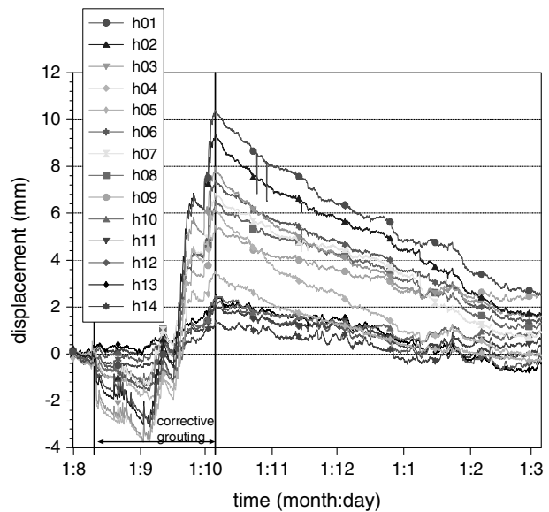
Figure 8. Heave and settlement as a function of time.
