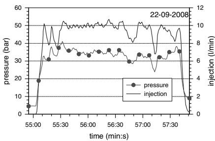
Figure 6. Example of a registration with a high injection pressure.
