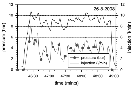
Figure 5. Example of a registration with a low injection pressure.
