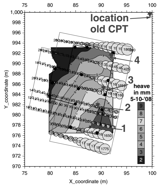
Figure 3. Overview corrective grouting at Vijzelgracht, see also text.
