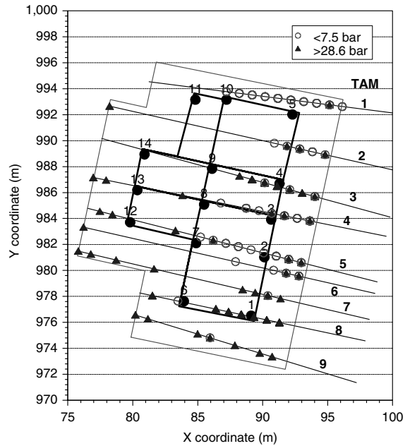
Figure 7. Locations where low and high injection pressures were found.
