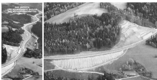
Fig..2. Situation after first phase of anchor installation 1985
