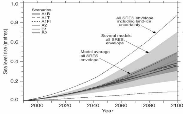
Fig.3 SLR (IPCC, 2001)
