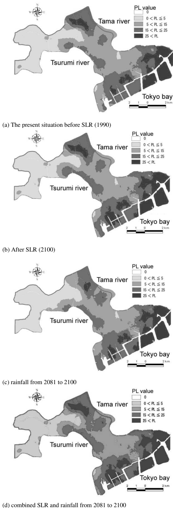
Fig.6 Liquefaction hazard maps
