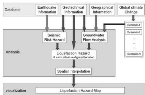
Figure 1. A procedure for liquefaction hazard mapping in consideration of global climate change
