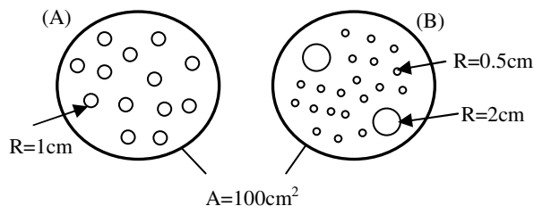
Figure 3. Models of soil columns with equal porosity ( n_A=n_B=0.41 ) and unequal permeability ( k_B=2.6 k_A ).
