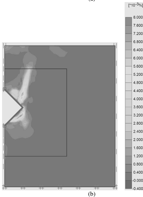
Figure 6. Contours of incremental shear strain: (a) parallel configuration; (b) 45° rotated configuration.
