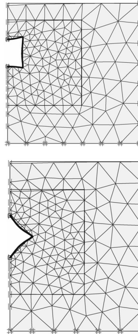
Figure 3. Geometry and finite element mesh for both culverts.
