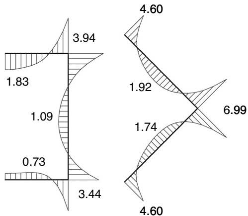
Figure 5. Bending moment diagrams for both culverts (kN.m/m)
