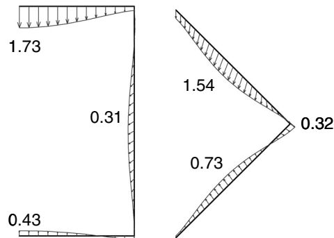
Figure 4. Total displacement diagrams for both culverts (m) ( \times 10^{-3} ).
