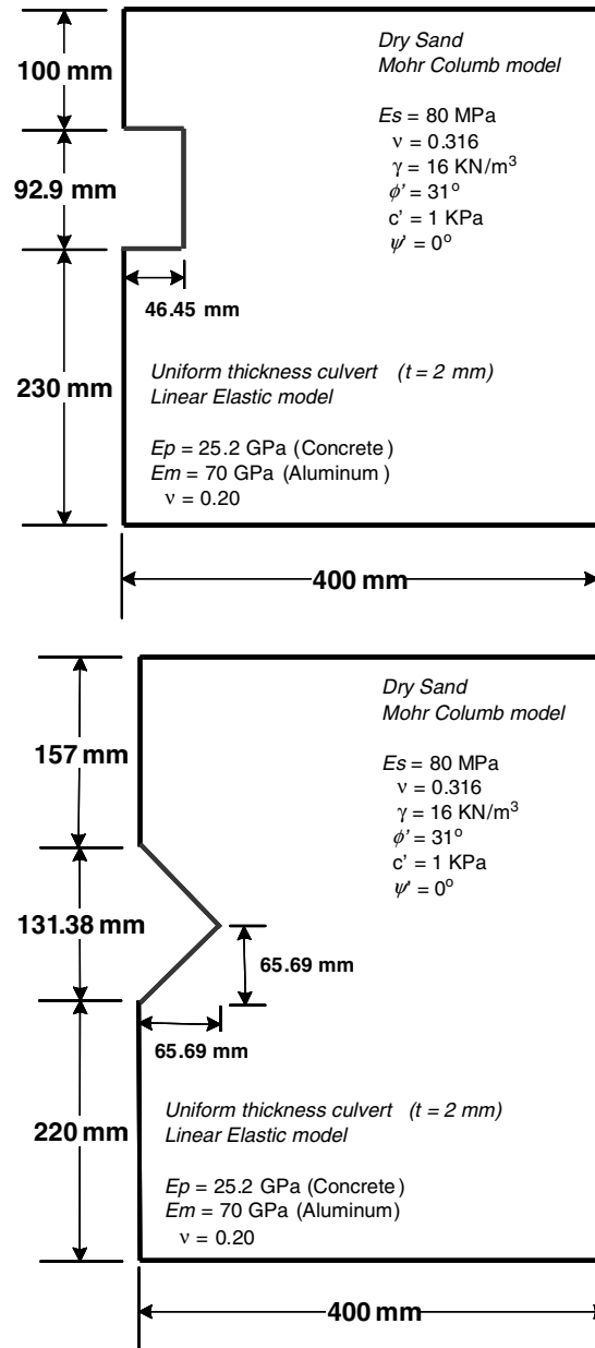
Figure 2. Schematic diagram showing the orientation of the two culverts and the properties used for analysis.
