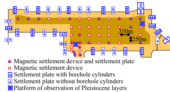
Figure 24. Arrangement plan of settlement measuring devices
