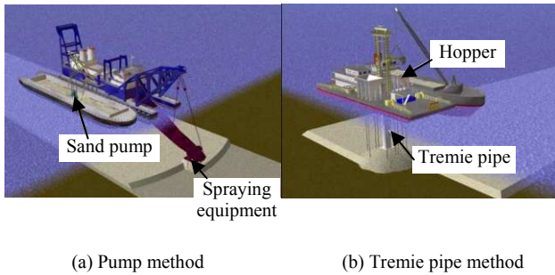
Figure 6. Methods of sand spreading
