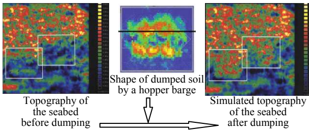
Figure 26. preliminary dumping simulation
