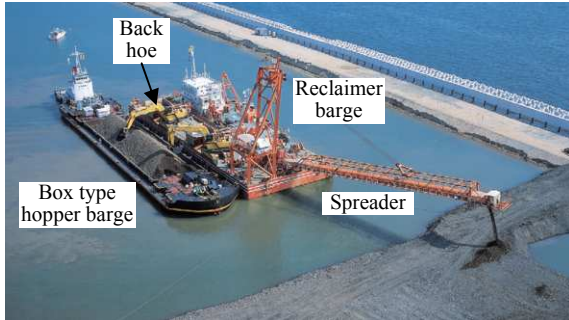
Figure 19. Reclaimer barge
