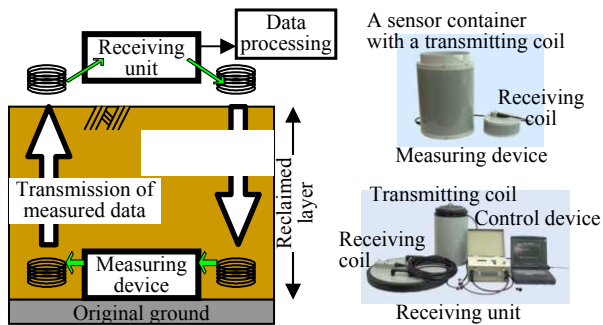
Figure 23. Hydraulic pressure gauge with a magnetic transmitter
