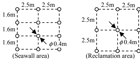
Figure 9. Spacing of sand drain piles
