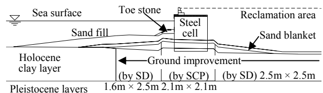
Figure 17. Typical cross section of the embedded-type steel cellular-bulkhead seawall
