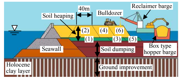
(1)~(6): Procedures of soil heaping work (1), (3), (5): Dumping-2 (2), (4), (6): Reclamation-1
