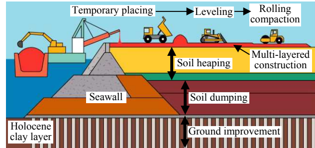
Figure 21. Progress of multi-layered construction
