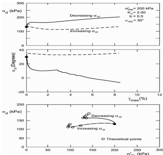
Fig. 11. Influence of the sense of principal stress rotation on initially non-axisymmetrically consolidated sand (after Sivathayalan and Vaid 2002)
