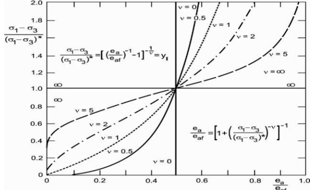
Fig. 2. Graphs of the pre-peak inverted function Y_I
