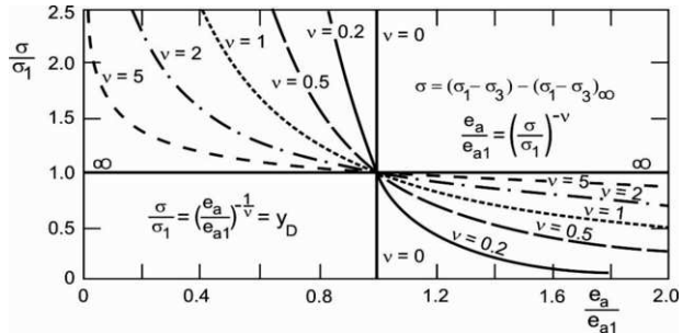
Fig. 3. Graphs of the post-peak ductility function Y_D
