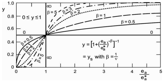
Fig. 4. Graphs of the sensitivity function Y
