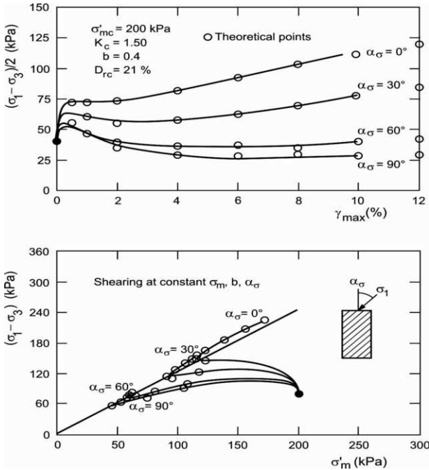
Fig. 6. Influence of the direction of major principal stress on the undrained behaviour at an initial static shear of K_c = 1.50 . \gamma_{max} , maximum shear strain (after Sivathayalan and Vaid 2002).
