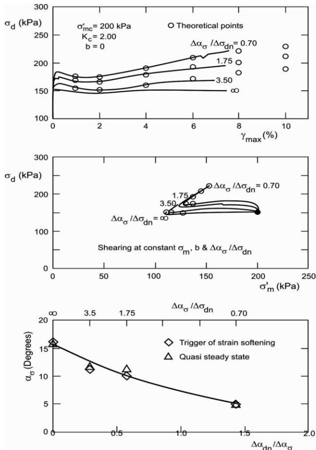
Fig. 9. Influence of the degree of stress rotation on the undrained response of sands at a given initial state (after Sivathayalan and Vaid 2002).
