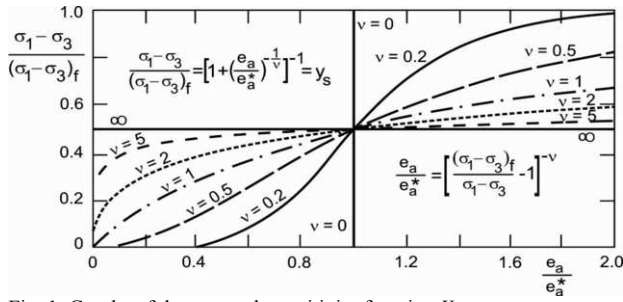
Fig. 1. Graphs of the pre-peak sensitivity function Y_s
