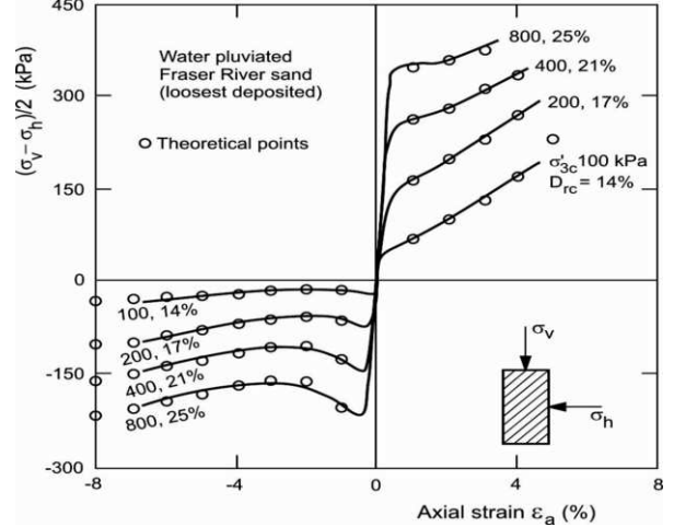
Fig. 5. Evidence of inherent anisotropy in undrained triaxial tests (after Vaid and Thomas, 1995). D_{rc} relative density at the end of consolidation; \sigma_h and \sigma_v horizontal and vertical stress, respectively.
