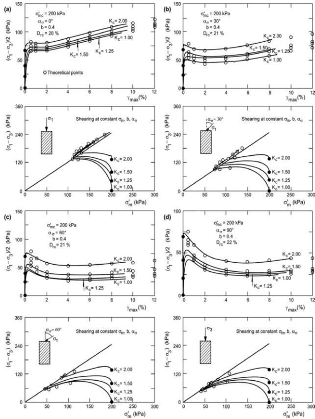
Fig. 7. Influence of initial static shear on the undrained behaviour of sands consolidated to \alpha_c = 0^\circ (a), 30^\circ (b), 60^\circ (c), and 90^\circ (d) (after Sivathayalan and Vaid 2002)
