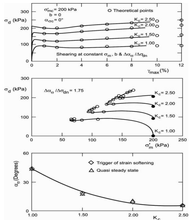
Fig. 8. Influence of initial static shear on undrained shear with principal stress rotation (after Sivathayalan and Vaid 2002)
