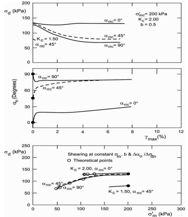
Fig. 10. Influence of initial static shear and principal stress direction on deformation due to principal stress rotation alone (after Sivathayalan and Vaid 2002).
