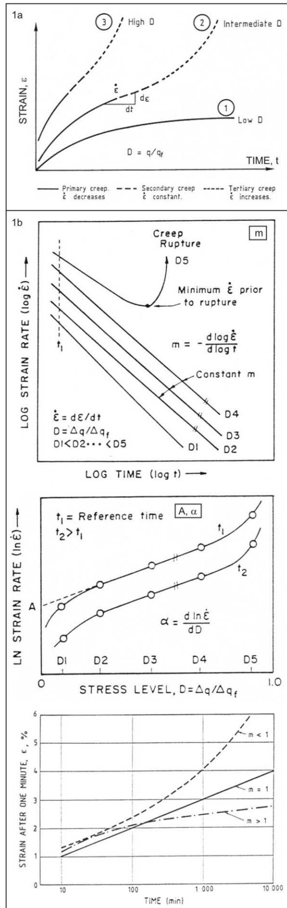
Figure 1. Basic creep behaviour from constant stress undrained creep testing on soft clays (after Mitchell, 1976)
