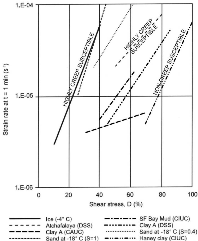
Figure 4. Creep susceptibility diagram
