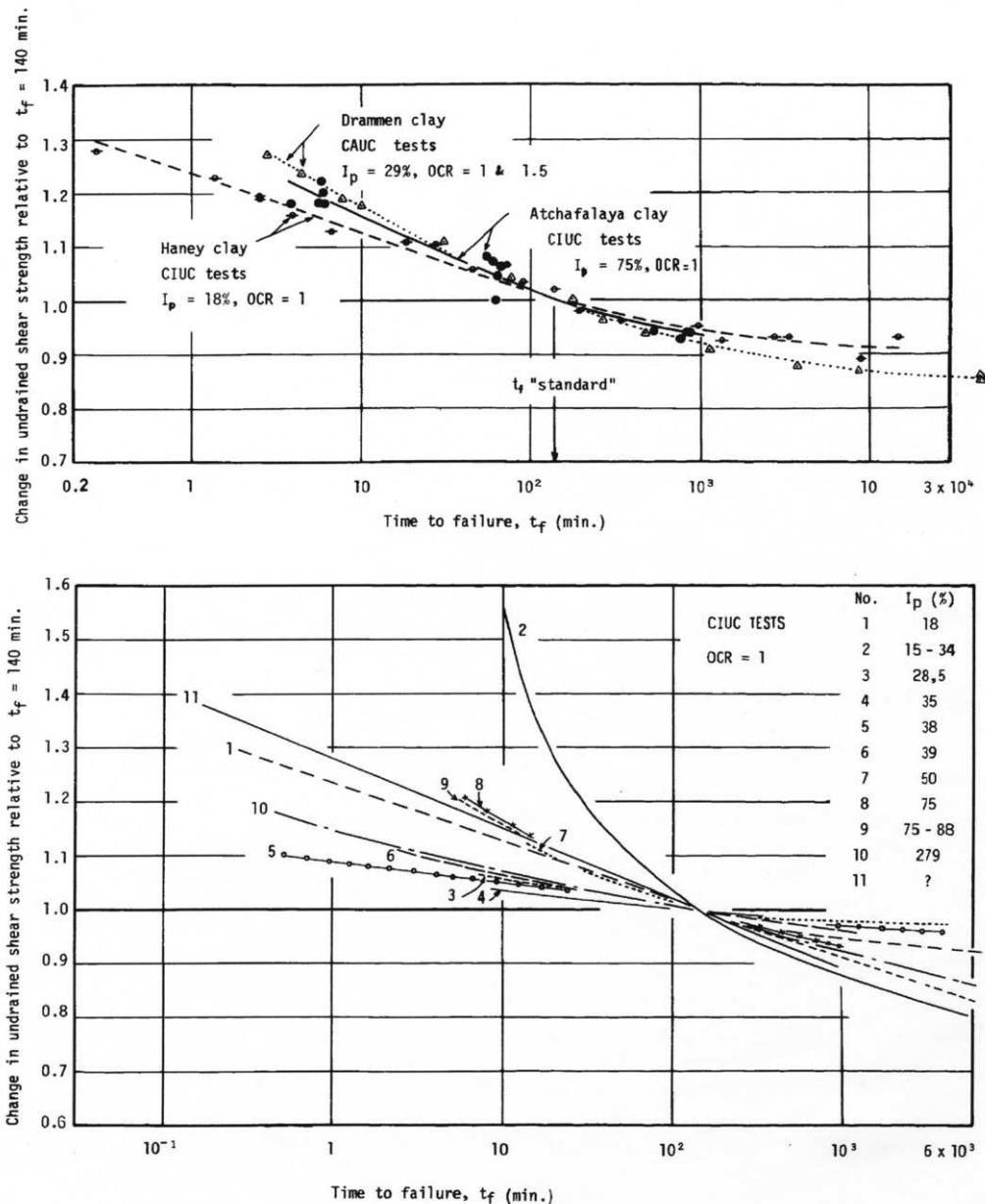
Figure 3. Effect of time to failure on undrained shear strength of normally consolidated clays (Lacasse, 1995).
