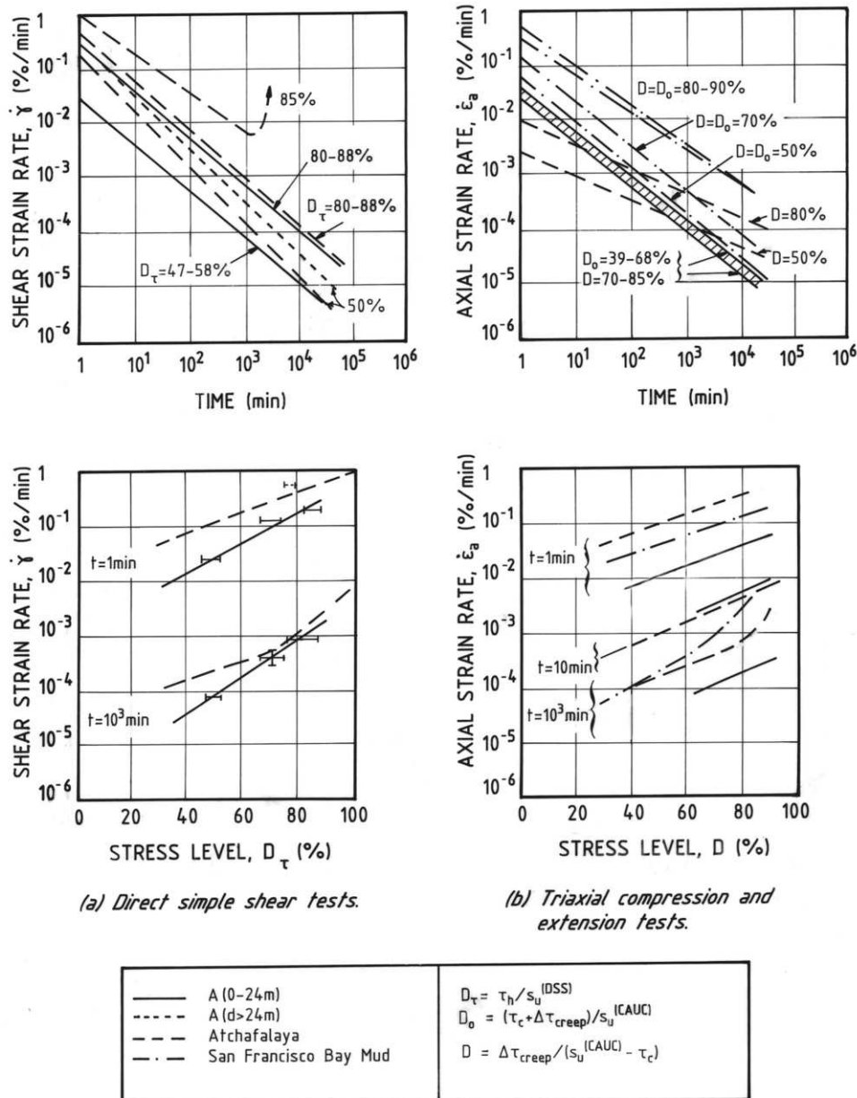
Figure 2. Results of triaxial and simple shear undrained creep tests on three clays.
