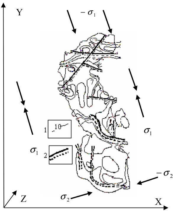
Figure 1. Scheme of isodepth of Sedimentary Cover Base (Lebedev L.I., 1987) 1— isohypses of sedimentary cover base, km.; 2— abyssal fracture
