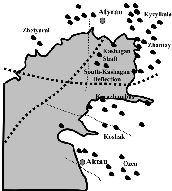
Figure 2. Scheme of location of oil and gas structures of the Kazakh sector of the Caspian Sea and its surroundings. 1— oil, oil and gas, gas and oil fields; 2 — local fractures; 3 — main fracture
