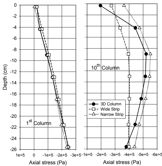
Figure 5. Axial stress of columns
