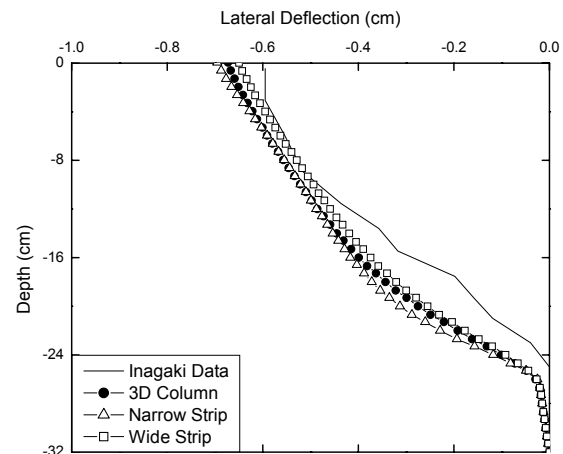
Figure 2. Deflections for analyses with five columns
