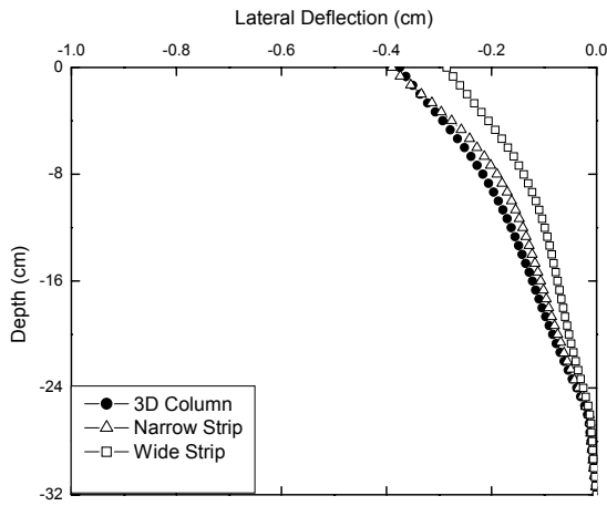
Figure 3. Deflections for analyses with ten columns
