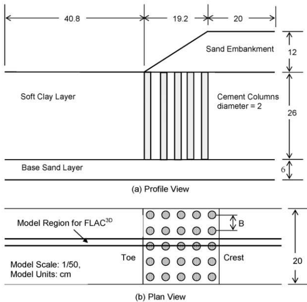
Figure 1. Inagaki et al. (2002) Centrifuge Model Schematic
