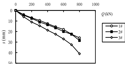
Figure 3. Q - s curves of DMM composite foundation
