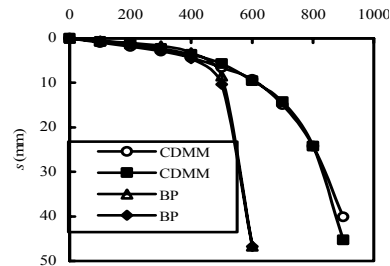
Figure 8. Q - s curve ( L=10.0m )
