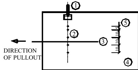
Fig. 2 a) specially instrumented GFOS pullout device, b) set up for measurement of wave velocity in the soil.
