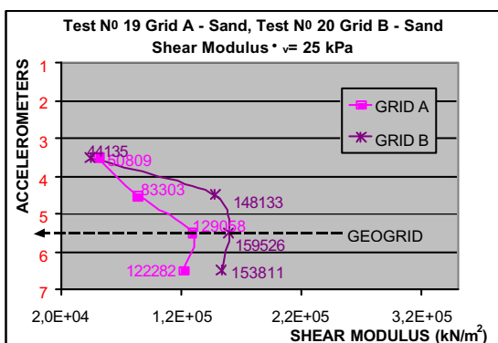
Fig.1. Measured G modulus distribution around two types of grid in sand using shear wave propagation method (distance between measuring points is 10 cm, results correspond to zones between them, Mulabdic et al, 2003)
