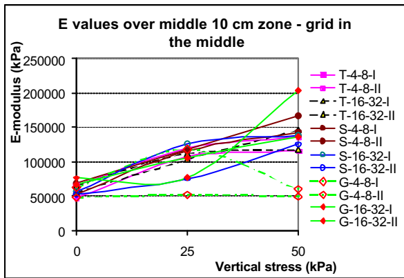
Fig.5. Development of the E modulus in the region of 10 cm around grid (T = Tensar SS30 grid, S = Secugrid 30/30, G = gravel, no grid, 48 mm = aggregate, 16-32 = aggregate, I, II = 1 st and 2 nd test)
