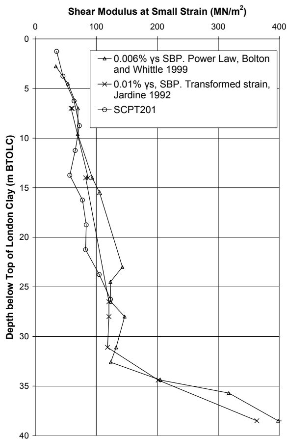
Figure 2: Shear Modulus at Small Strain vs Depth Below Top of London Clay ( \gamma_s = shear strain)
