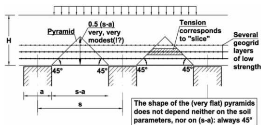
Figure 3. The so-called “Guido Method”
