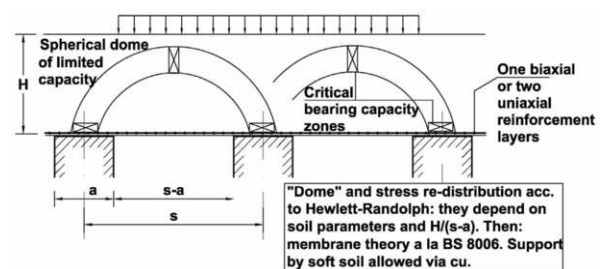
Figure 6. The “Older German Method”
