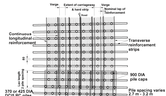
Figure 11. A 63 Selby Bypass: typical layout of reinforcement
