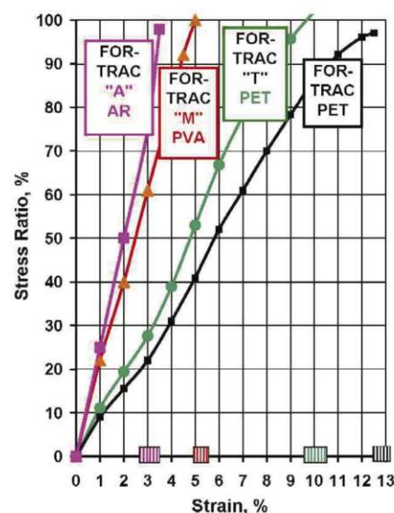
Figure 2. Influence of the polymer used on the tensile force-strain behavior of similar geogrid “families”
