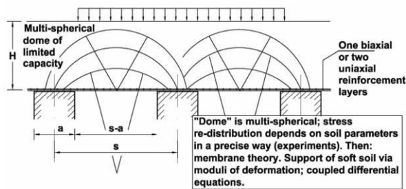
Figure 7. The “New German Method”
