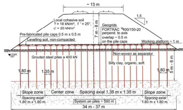
Figure 9. Typical cross-section Crossing “River Laje”
