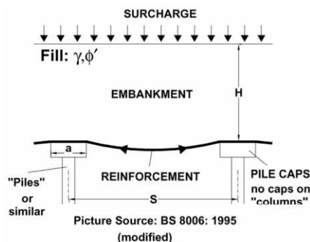
Figure 1. General idea of reinforced embankments on piles
