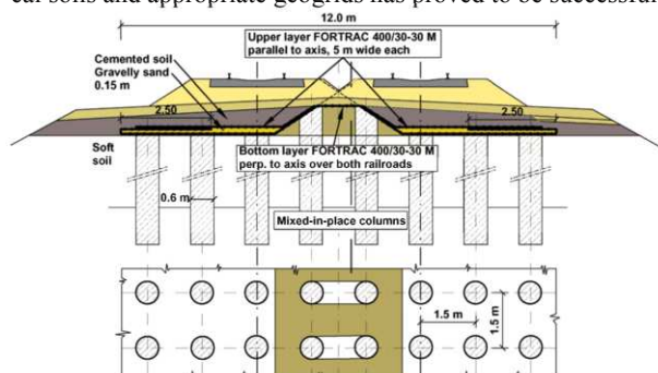
Figure 13: Typical cross-section “Büchen”; the bottom geogrid is installed over the entire width, the upper ones separately in the left and right half
