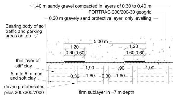
Figure 8. Cross-Section “Shell-Station” in Sofia
