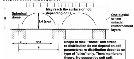
Figure 5. The “BS 8006 Method”
