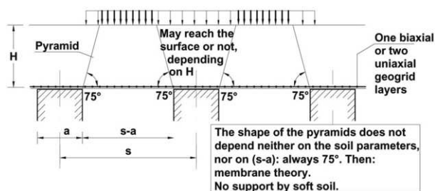
Figure 4. The “Swedish Method”
