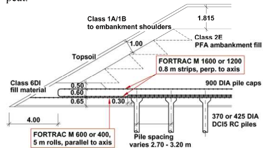
Figure 10. A63 Selby Bypass: typical cross-section
