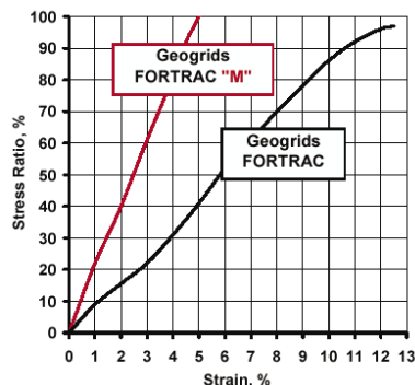
Figure 12: A 63 Selby Bypass typical normalized stress-strain curves for the geogrids used
