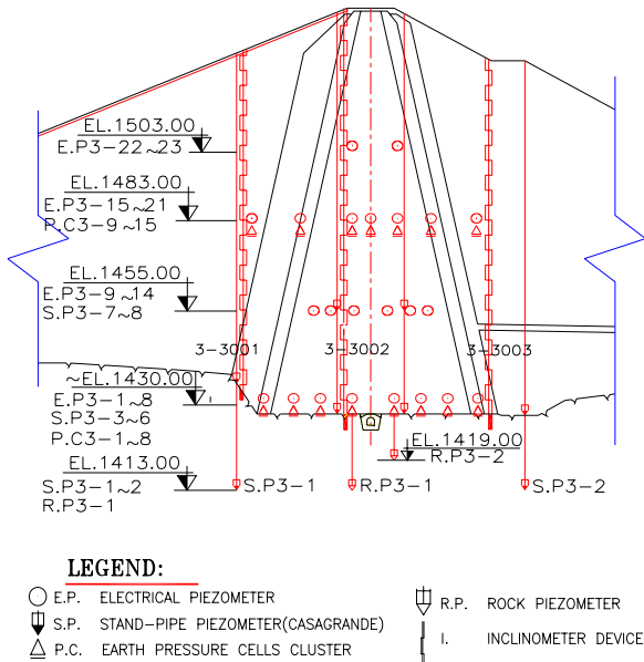
Figure 2. Transverse third instrumented section
