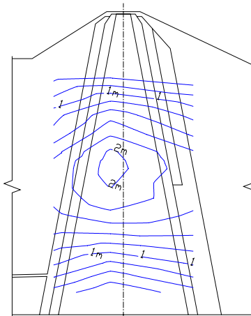
Figure 3. Pttren of vertical displacement
