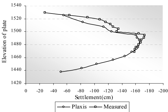
Figure 9. Settlement plates positioning in downstream of clay (Feb 2003)
