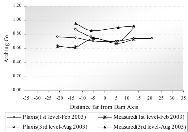
Figure 15. Arching coefficient in clay in 1 st and 3 rd level of installation
