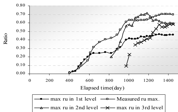
Figure 12. Maximum ratio of pore water pressure in clay
