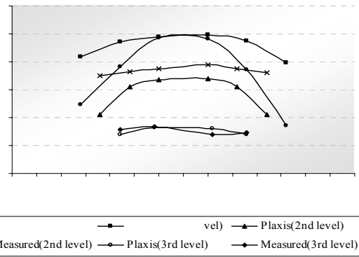
Figure 11. Pore water pressure in clay in 1 st , 2 nd and 3 rd level of installation (last reading-Feb 2003)
