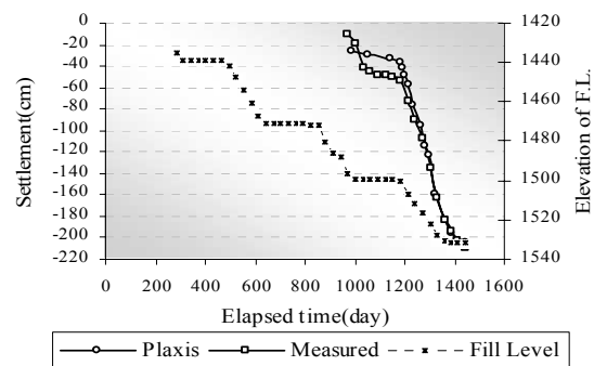
Figure 4. Settlement plate positioning (20 th ) in clay, elevation of installing: 1494.17
