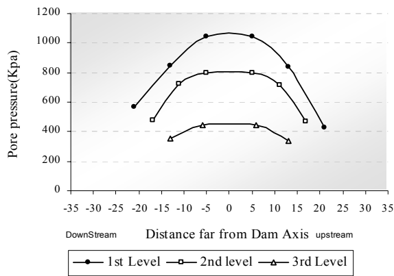
Figure 13. Predicted pore water pressure in clay in end of construction
