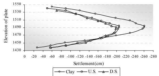
Figure 10. Predicted settlement in dam body in end of construction
