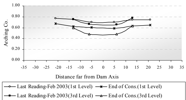
Figure 16. Predicted arching coefficient in clay in 1 st and 3 rd level of installation
