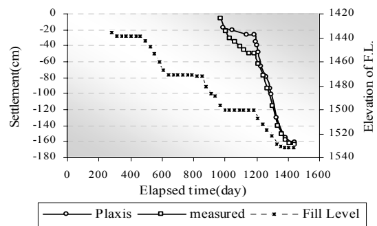
Figure 5. Settlement plate positioning (20 th ) in upstream of clay, elevation of installing: 1494.28
