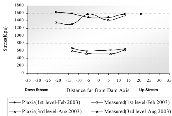
Figure 14. Vertical total stress in clay in 1 st level, 1430 masl and 3 rd level, 1483 masl, of installation
