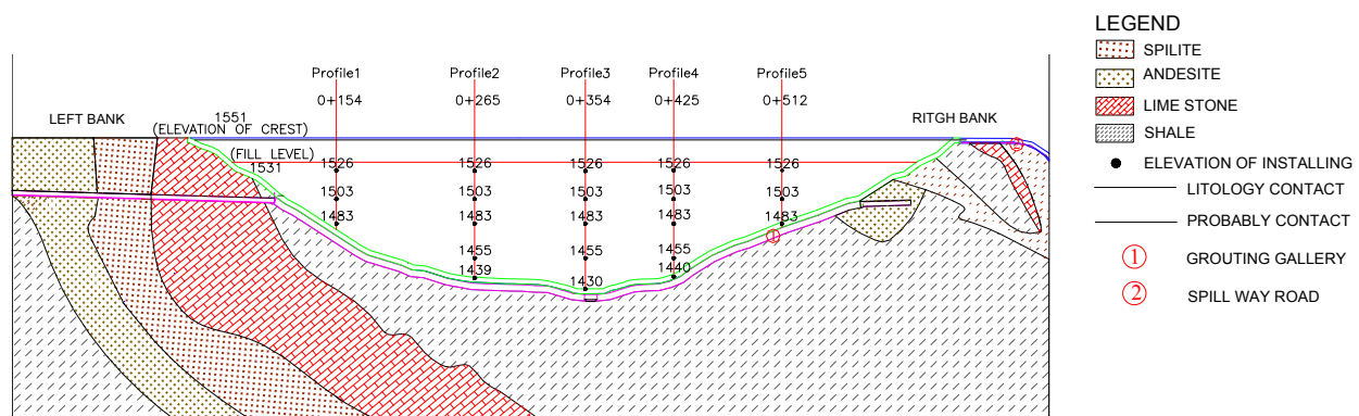
Figure 1. Longitudinal section of dam body
