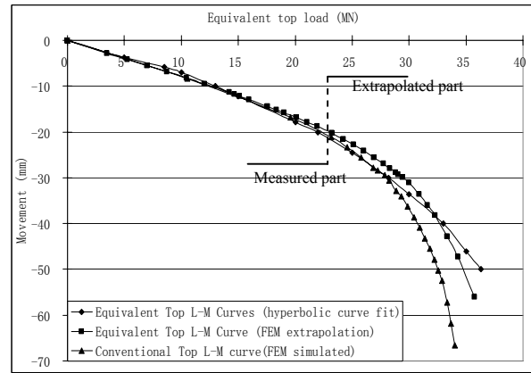
Figure 9. Equivalent top load-movement curves.
