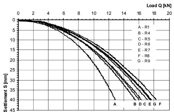
Figure 5 The comparison between averaged load-settlement relations.
