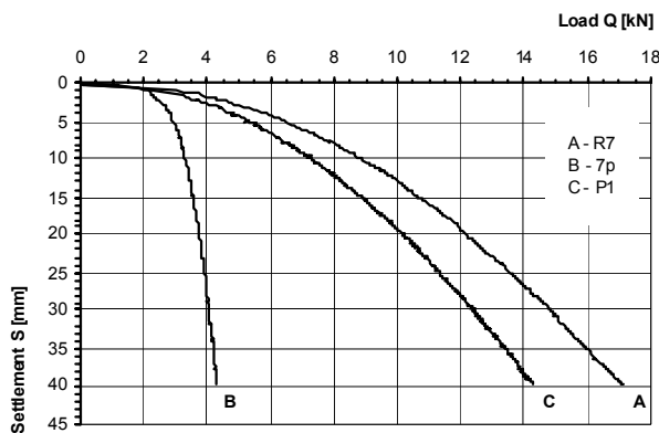
Figure 6 Load-settlements curves for 7 piles' scheme.
