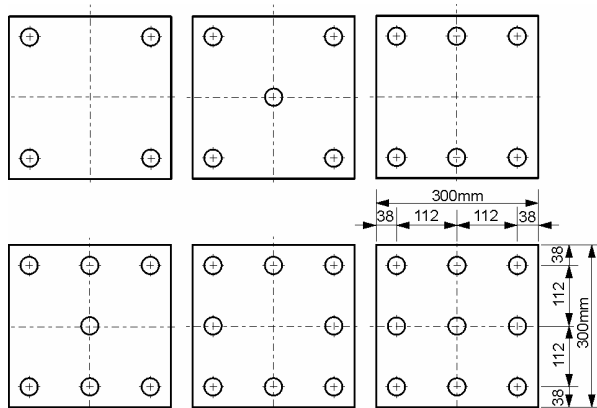
Figure 3 Schemes of various sets of pile groups and piled raft foundations.
