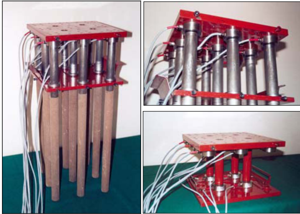
Figure 2 Piled raft foundation model.
