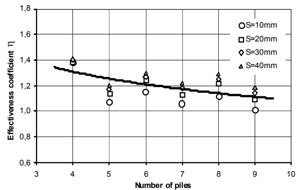
Figure 9 Effectiveness coefficient \eta of piled raft foundation
