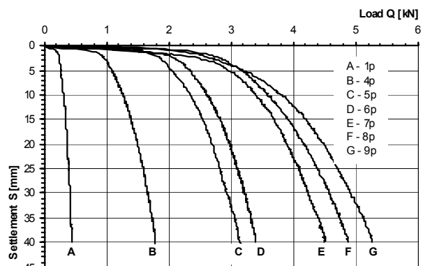
Figure 4 Load-settlement relations for groups of piles.
