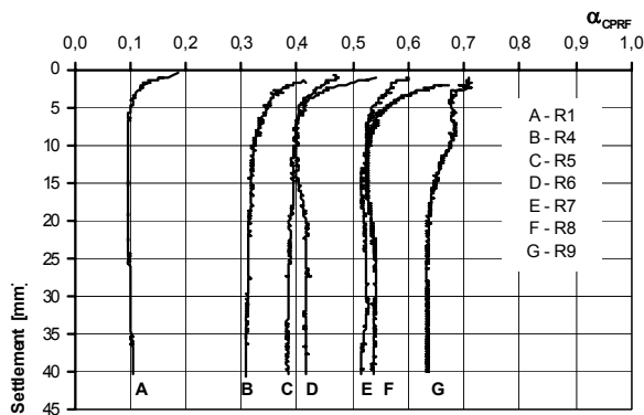
Figure 8 \alpha_{CPRF} ratio determined by model tests.
