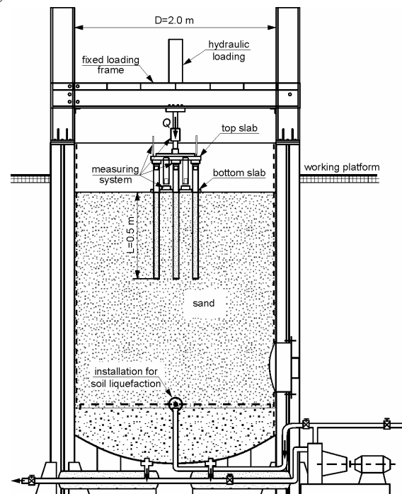
Figure 1 Scheme of lab stand for wet non-cohesive soil.
