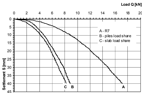
Figure 7 Contribution of slab and piles in transmission of loads into the subsoil. Slab on 7 piles.
