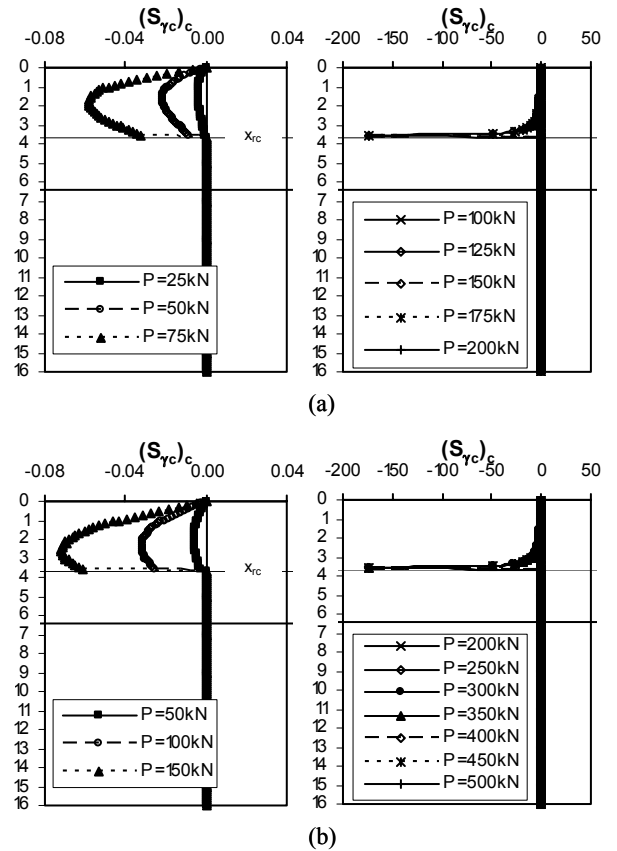
Figure 6. Distribution of (S_{\gamma'_c})_c for (a) free head pile (b) fixed head pile
