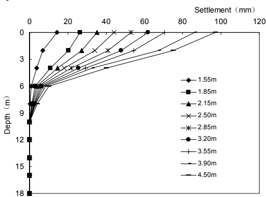
Fig.5 Settlement at Various Depths at K12+592
