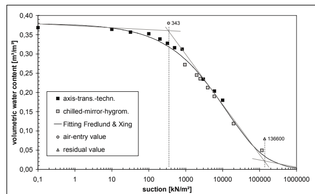
Figure 3. Soil-water characteristic curve of clay Plessa (PI1000), fitted with Fredlund & Xing (1994)
