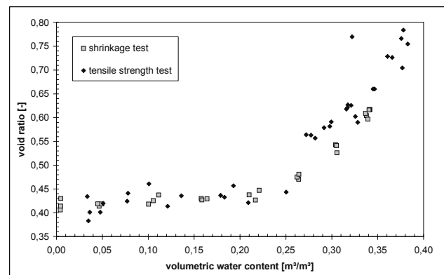
Figure 2. Shrinkage curve of clay Plessa (PI1000)
