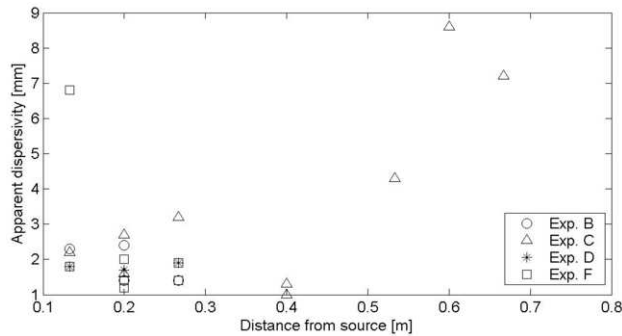
Figure 4 : Results of two-well tracer tests.
