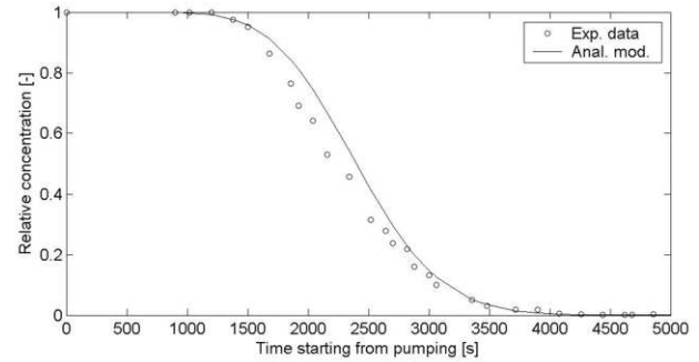
Figure 5 : Concentration recovery during single-well test.
