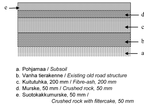
Figure 3: Principle of a fibre-ash structural course –system (Kukkia Circlet, Pilot 2003)
