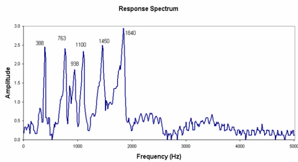
Figure 2 Axial response spectrum obtained on composite laboratory nail using medium instrumented hammer
