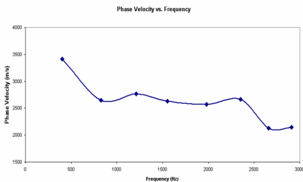
Figure 4 Phase velocities for the first eight modes calculated using experimentally obtained modal phases
