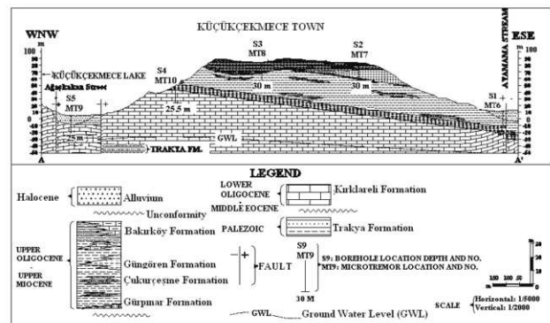
Figure 2. The geological cross-section (A-A') of the region
