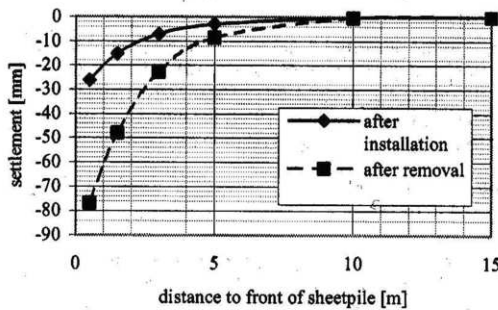
Fig. 6 Settlements induced by sheet pile installation and extraction ( Meijers and van Tol 2005 )
