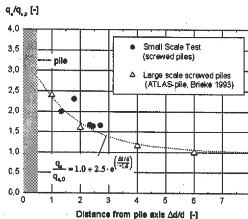
Fig. 1. Increase in CPT q_c resistance adjacent to a screw pile (reproduced from Katzenbach & Schmitt 2005 )
