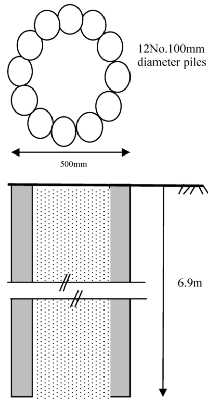
Fig.3. Creation of a large diameter pipe pile using small diameter jacked piles ( Deeks et al. 2005 )
