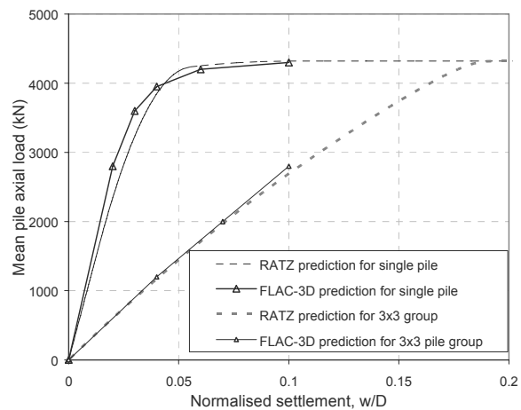
Fig. 7 Comparison of FLAC-3D analyses of Comodromos & Bareka (2005) with predictions using RATZ for a 3 \times 3 pile group ( s/D=3 , L/D=25 )
