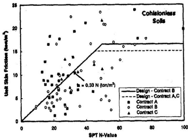
Fig. 4. Backanalysed correlation between the SPT N value and shaft friction on bored piles in sand (reproduced from Seah et al. (2005) ).
