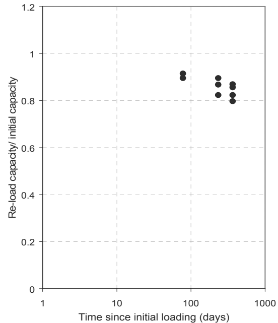
Fig. 10. Reload shaft capacity of bored piles in London Clay (reproduced from Unwin & Jessep 2004)
