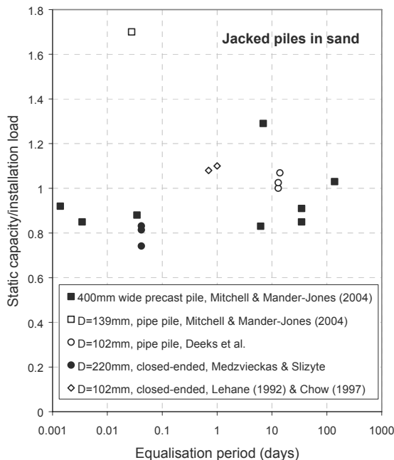
Fig. 2. Ratio of static compressive capacity to installation capacity of jacked piles in sand
