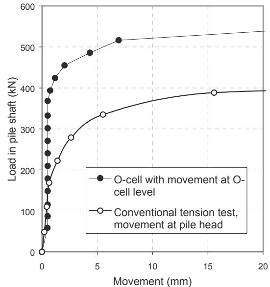
Fig. 9. Comparison of Osterberg-cell test with an equivalent conventional static tension test (Kumar et al. 2004).
