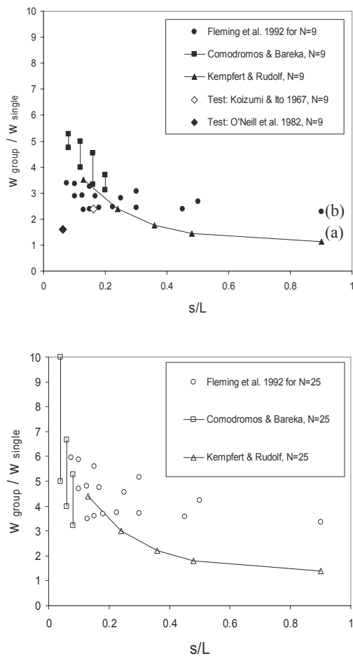
Fig. 8. Pile group settlement ratios for (a) 3 \times 3 pile group and (b) 5 \times 5 pile group
