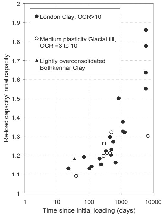
Fig. 9. Gain in capacity on re-loading of displacement piles in clay (reproduced from Powell et al. 2003)
