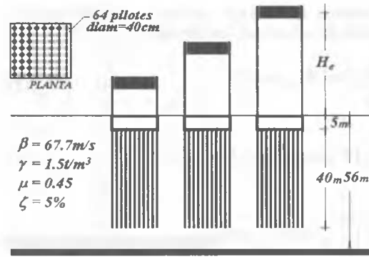
Figure 6. Soil-foundation-structure system
