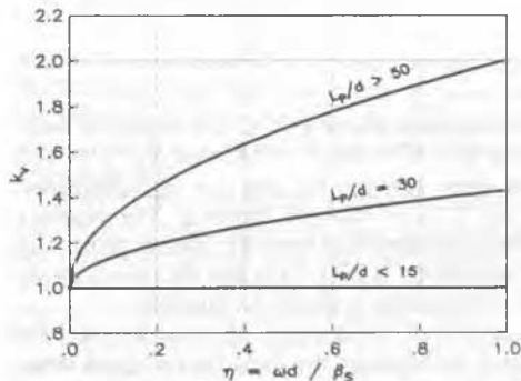
Figure 5. Stiffness coefficients for floating pile on Mexico City under vertical vibrations.
