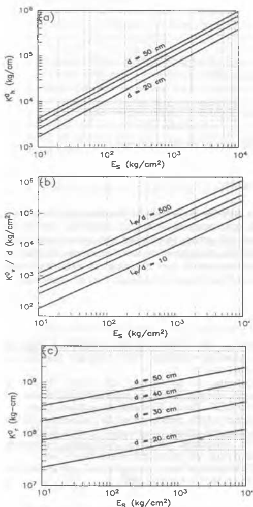
Figure 3. Static stiffness for floating pile on Mexico City under horizontal (a), vertical (b) and rocking (c) vibrations.
