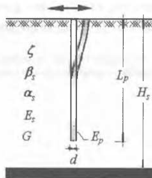
Figure 2. Floating pile under horizontal vibrations.
