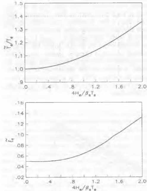
Figure 7. Effective structural period and damping
