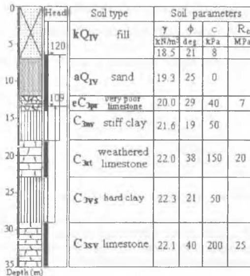
Figure 2. Typical soil profile.
