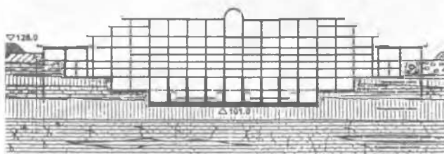
Figure 4. Cross section of the Central Mall.
