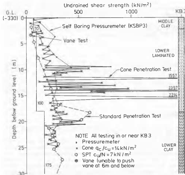
Figure 2 Comparison of insitu undrained strength
