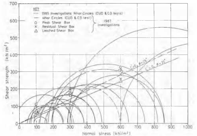
Figure 3 Mohr Circles for effective Stress, Middle Clay
