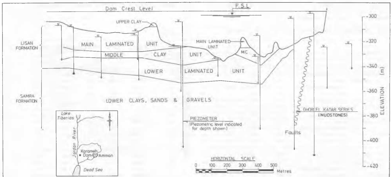
Figure 1 Cross section along dam centreline
