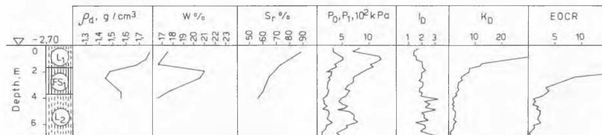
Fig. 2 Soil Data and Dilatometer Test Results at Russe, Site 1, Compacted Loess
