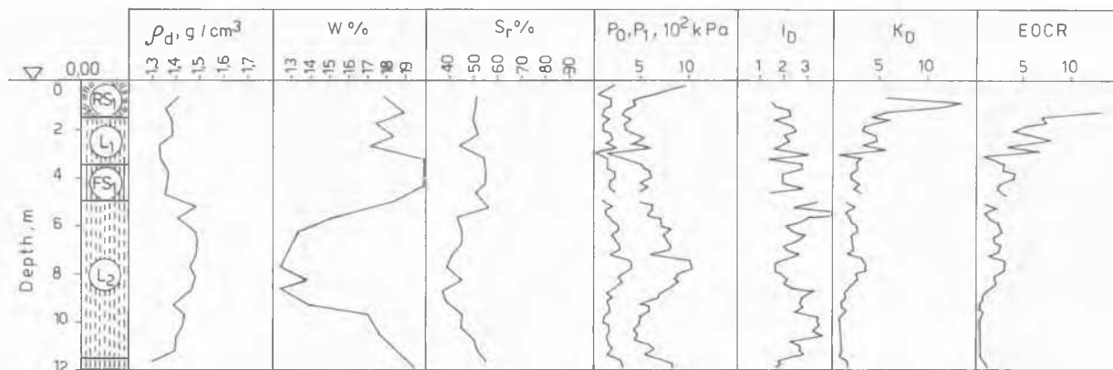
Fig. 3 Soil Data and Dilatometer Test Results at Russe, Site 2, Natural Loess
