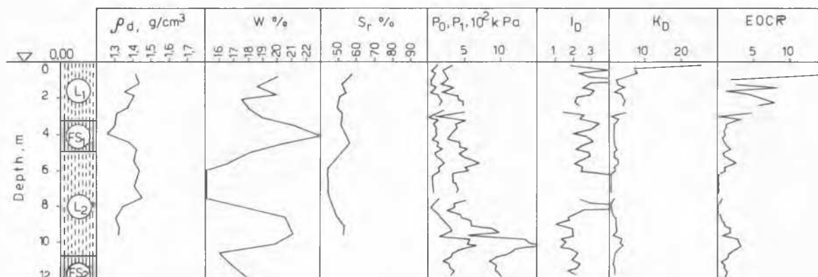
Fig. 1 Soil Data and Dilatometer Test Results at Russe, Site 1, Natural Loess
