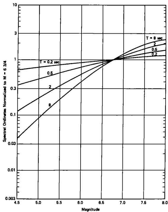
Revised Fig. B-5 Approximate Dependence of Spectral Ordinates on Magnitude -- Results Normalized with Respect to m=6-3/4
