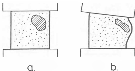
Fig. 10 Heterogeneous specimen
