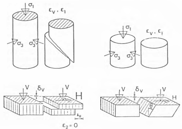
Fig. 1 Some specimens before and after testing. Fixed ends are hatched
