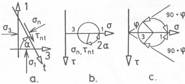
Fig. 2 Mohr's circle for stresses
