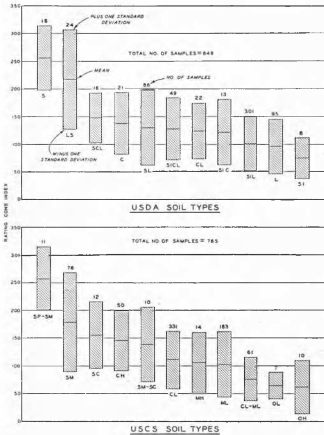
Fig. 5 Rating cone indexes at field maximum moisture contents, means and ranges.
