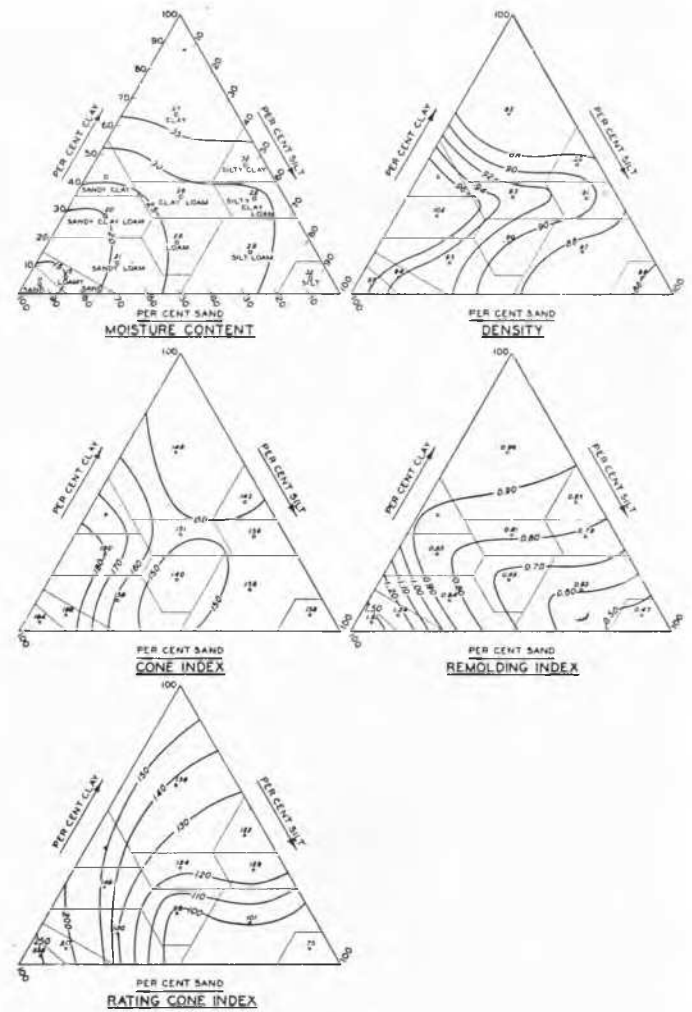
Fig. 6 Mean values of soil properties at field maximum moisture contents.
