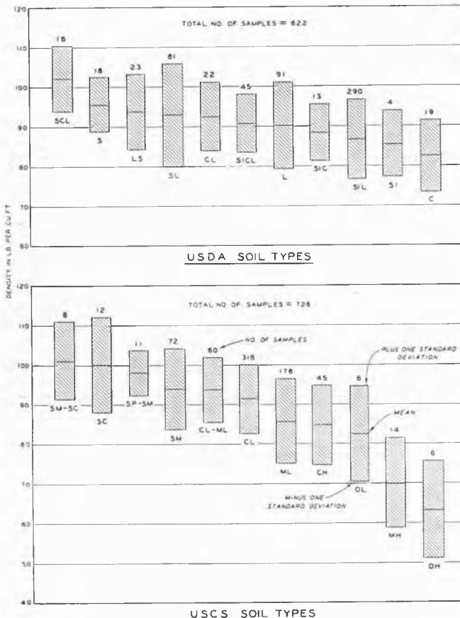
Fig. 2 Densities at field maximum moisture contents, means and ranges.
