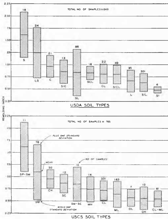
Fig. 4 Remolding indexes at field maximum moisture contents, means and ranges.
