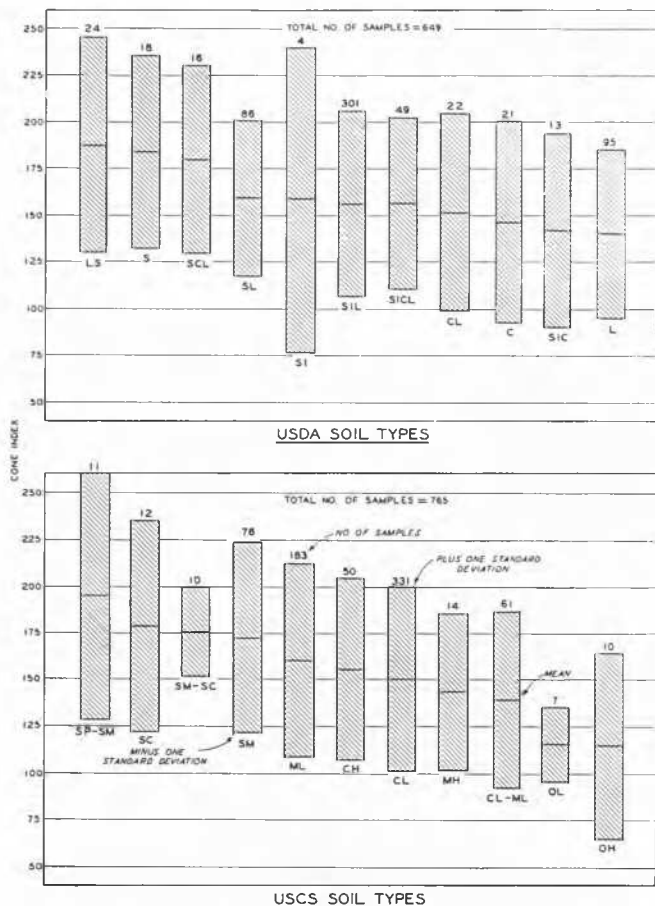
Fig. 3 Cone indexes at field maximum moisture contents, means and ranges.
