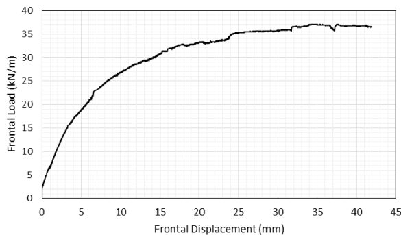
Figure 2. Frontal pullout load-displacement behavior
