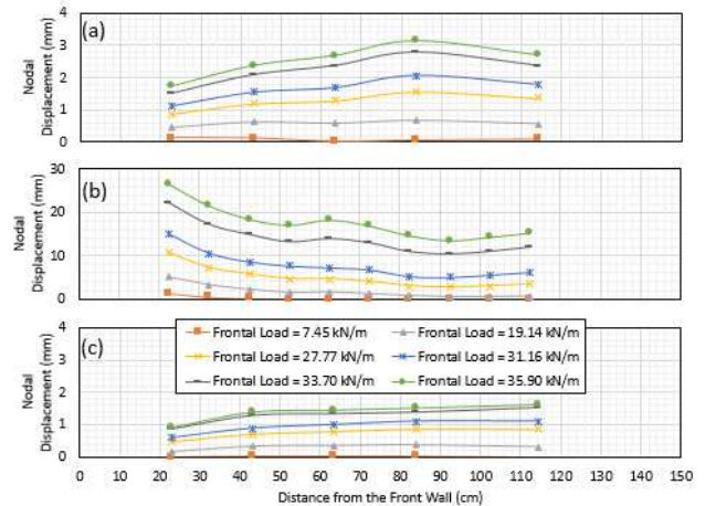
Figure 3. Reinforcement nodal displacement: (a) Main layer; (b) Upper boundary layer; and (c) Bottom boundary layer
