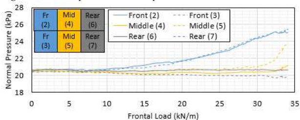
Figure 6. Normal pressure on the top of the reinforced soil mass
