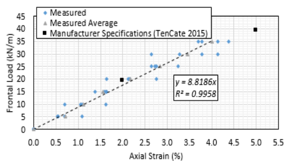
Figure 7. Reinforcement unconfined tensile behavior
