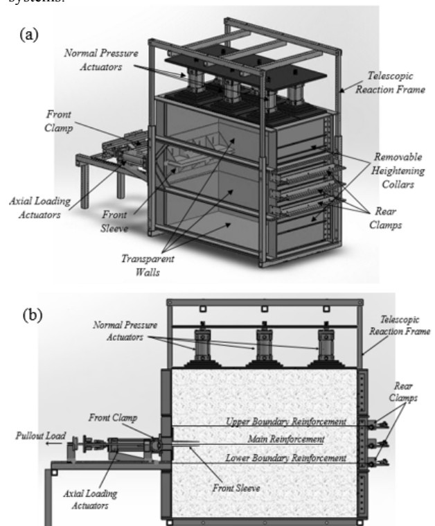
Figure 1. General layout of the new equipment: (a) 3D perspective; (b) sectional side view.
