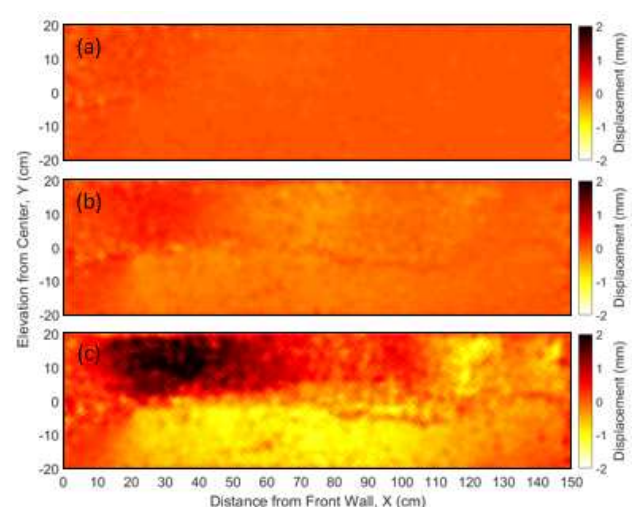
Figure 5. Vertical displacement field: (a) at 7.4-kN/m frontal load; (b) at 19.1-kN/m frontal load; (c) at 35.9-kN/m frontal load
