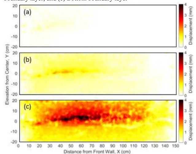
Figure 4. Horizontal displacement field: (a) at 7.4-kN/m frontal load; (b) at 19.1-kN/m frontal load; (c) at 35.9-kN/m frontal load
