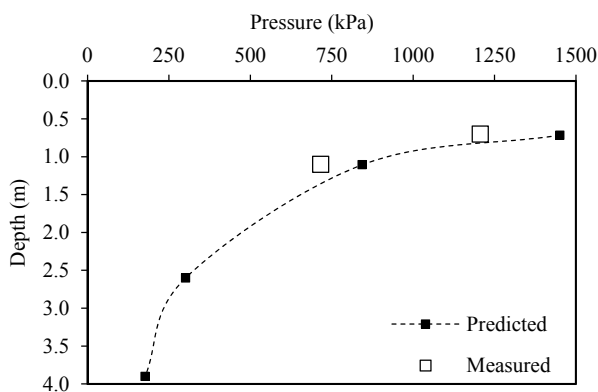
Figure 9. Predicted pressures from model compaction versus measured pressures from full size impact roller.
