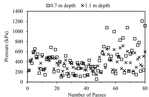
Figure 7. Measured peak pressure for each pass of the BH-1300 impact roller during field testing.
