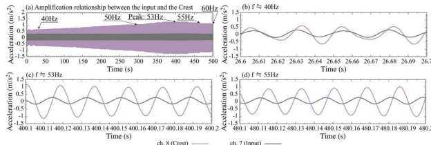
Figure 2 Result of the sweep test (relationship between input and measured acceleration amplitude)
