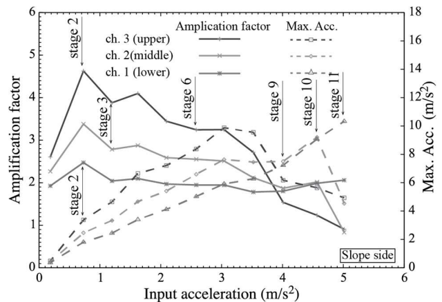
Figure 3 The measured acceleration and corresponding change in amplification factor
