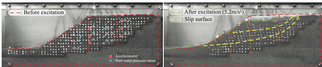
Photograph 1 Side view of the model prior to excitation and at step 11 (input acceleration of 5.2 m/s 2 ).
