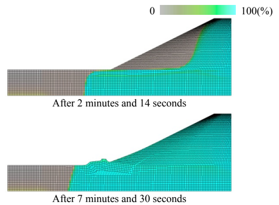
Figure 6. Calculation results for contours of degree of saturation (the covering soil layer is No. 8 sand)
