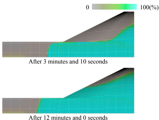
Figure 9. Calculation results for contours of degree of saturation (the covering soil layer is No. 8 sand, and the water level is low at 210 mm)
