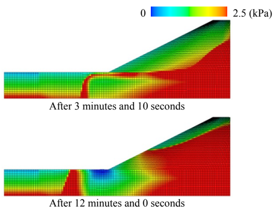
Figure 11. Calculation results for contours of mean skeleton stress (the covering soil layer is No. 8 sand, and the water level is low at 210 mm)
