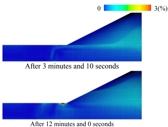
Figure 10. Calculation results for contours of shear strain (the covering soil layer is No. 8 sand, and the water level is low at 210 mm)
