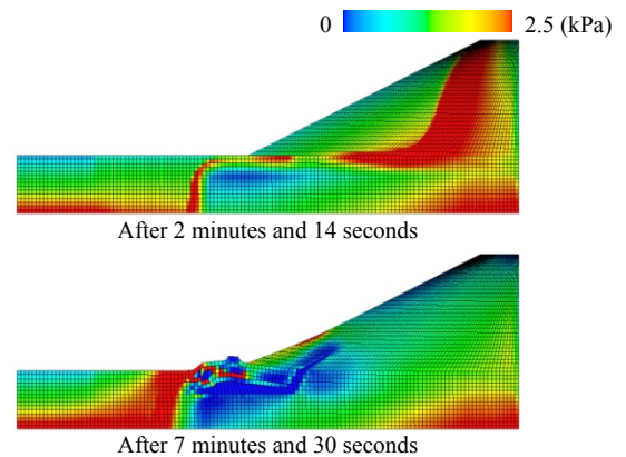
Figure 8. Calculation results for contours of mean skeleton stress (the covering soil layer is No. 8 sand)
