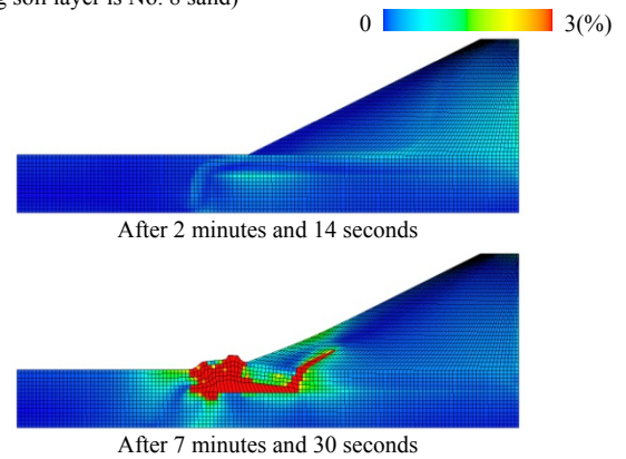
Figure 7. Calculation results for contours of shear strain (the covering soil layer is No. 8 sand)
