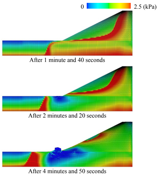
Figure 5. Calculation results for contours of mean skeleton stress
