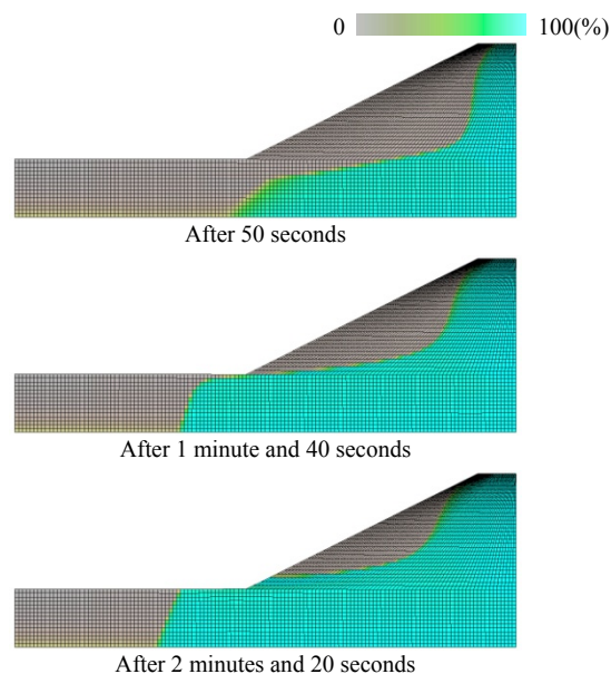
Figure 3. Calculation results for contours of degree of saturation
