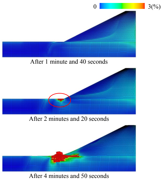
Figure 4. Calculation results for contours of shear strain
