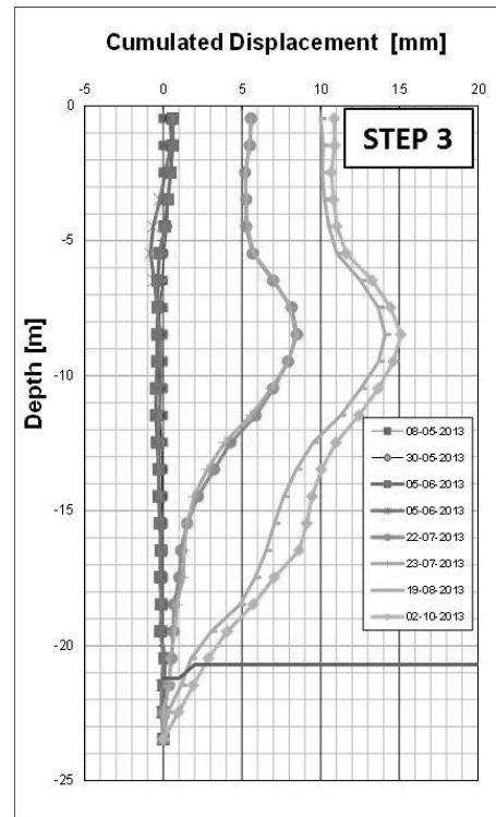
Figure 4. Horizontal deformations of stage 3.
