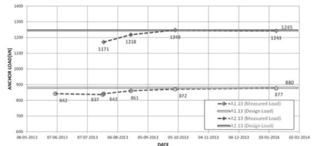
Figure 5. Measured ground anchor loads.
