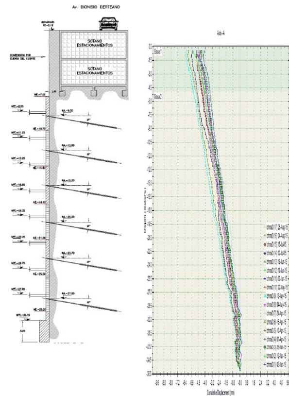
Figure 13. Cross-section of the wall and inclinometer readings.
