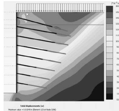
Figure 16. Open excavation completed.
