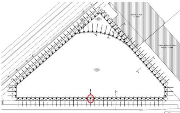
Figure 2. Excavation layout and monitored pile.
