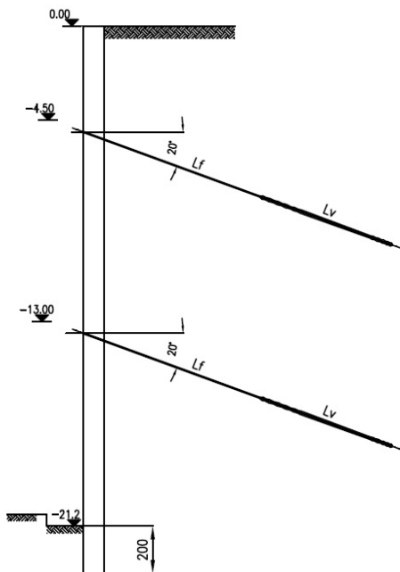
Figure 3. Cross section of the anchored pile wall.
