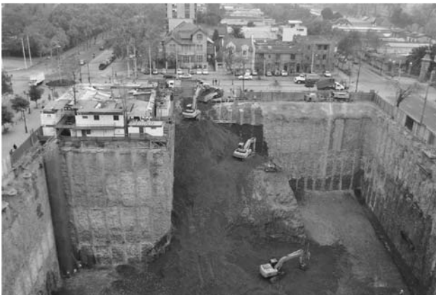
Figure 8. Deep excavation of 26.5m in Santiago, ramp withdrawal.
