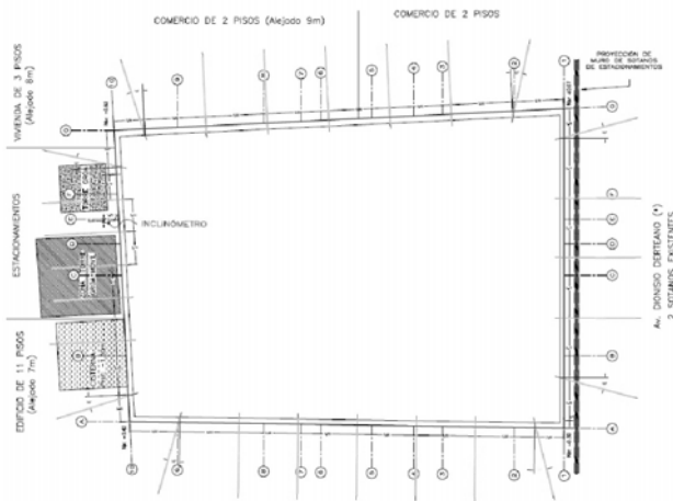
Figure 12. Excavation layout and monitored section on the left side.
